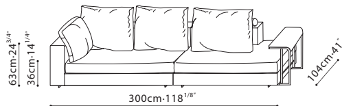
C0102203+C0102207+C8102201+C8102203x2 +C8102204+C0660001
