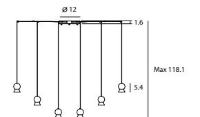
FUJI Pendant P12 SLD-1011PF12 LED 12 x 7W(3000K, CRI 90, 6600lm) Built-in dimmable driver Black PVC wire With hooks Materials : mouth-blown glass, steel Color : matt black Canopy : black
