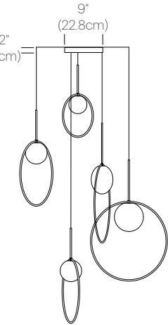
BOLA HALO MULTI-LIGHT 12, 18, 18, 22, 22
