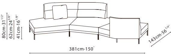
C01F0115+C01F0114x2+C81F0101
