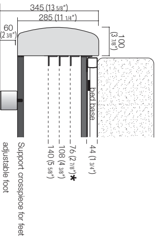
Bed frame section H 11 1/4"
