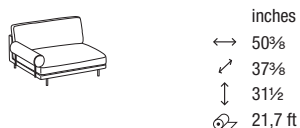
DTL1C0ES - DTL1C0ED 1-ER LATERAL EXTRA ELEMENT
