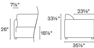
CS3469 with optional foot 2 3⁄8" H
