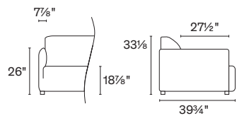
CS3469 /XP with optional foot 2 3⁄8" H
